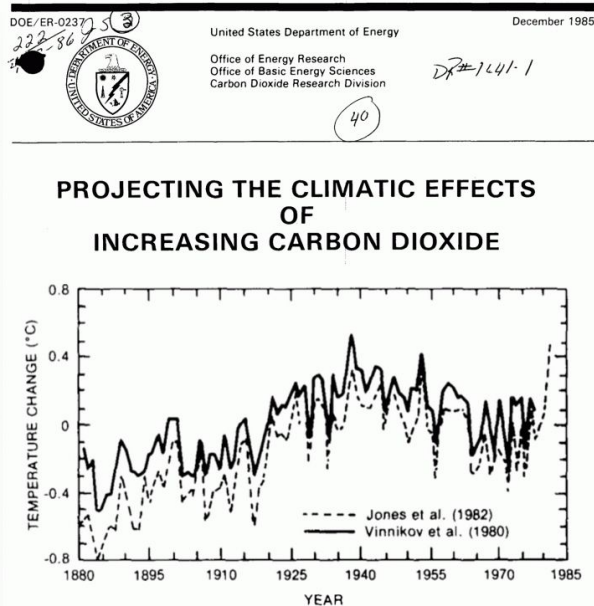
Figure 5.1. Annual mean surface air temperature anomalies from 1880–1981: (solid curve) Vinnikov et al. (1980); and (dashed curve) Jones et al. (1982). Figure from Weller et al. (1983), and includes points updated to 1981 by Jones.
