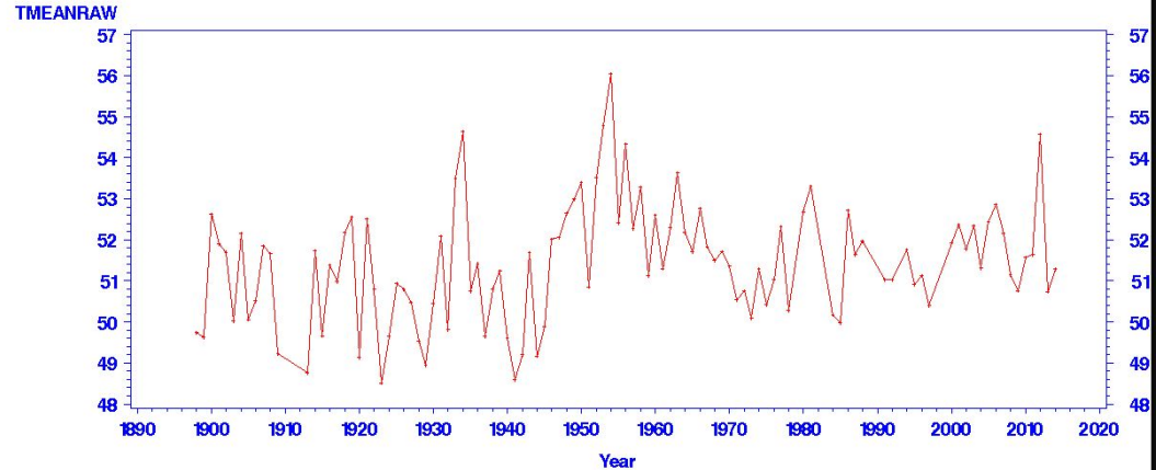
USHCN 050848, BOULDER, CO Annual mean of Monthly Mean Temperature -- RAW (F) 1893 -- 2014
